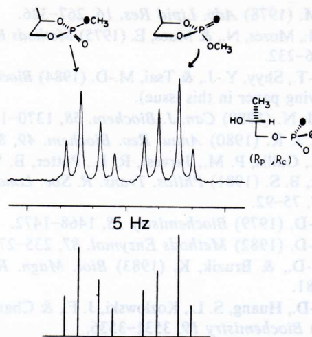
FIGURE 7: Observed and calculated ^{31}\text{P} NMR spectra ( \text{CD}_3\text{CN} , 121.47 MHz) of the cyclic triesters derived from [\text{}^{16}\text{O}, \text{}^{17}\text{O}, \text{}^{18}\text{O}] -phospho-( R )-propane-1,2-diol ( 16 ). Spectral parameters were as follows: spectral width 500 Hz, 16K data points, ^1\text{H} decoupling, 90^\circ pulse, line broadening 0.2 Hz, chemical shift +19.7 ppm, and temperature 25^\circ\text{C} .
